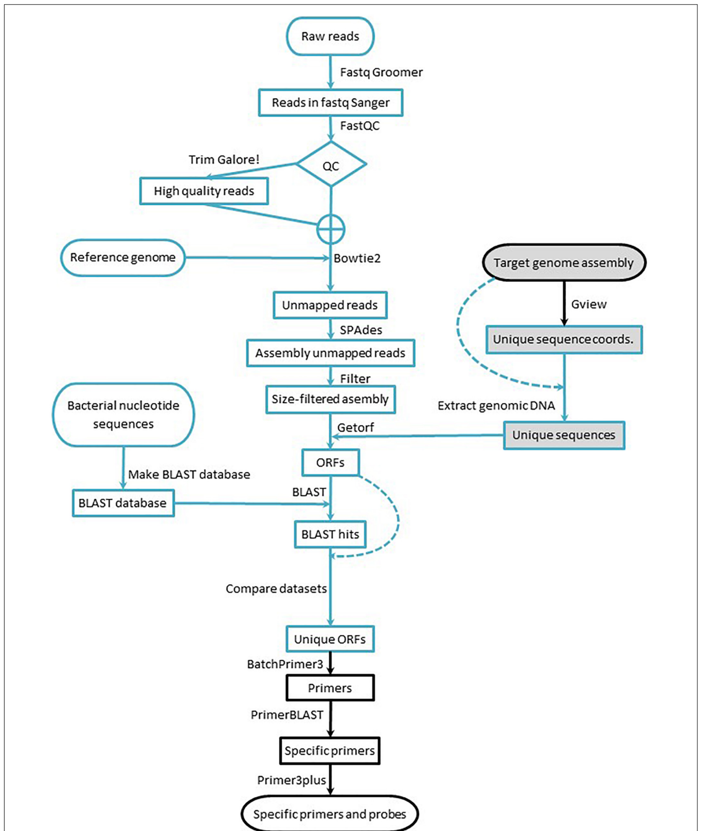
FIGURE 1 | Workflow for marker design. Blue lines indicate processes run in the Galaxy environment, and black lines indicate processes run using online tools. Arrows indicate the workflow direction, and dashed lines indicate processes that require a dataset for a second time. Shaded elements denote the part of the workflow applied to data acquired with long read sequencing technology.
